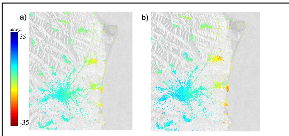
Figure 5. Velocities (1992-2000) of the broader area of Katerini (rectangle f. from Fig.3) a) SBAS method b) PS method.
