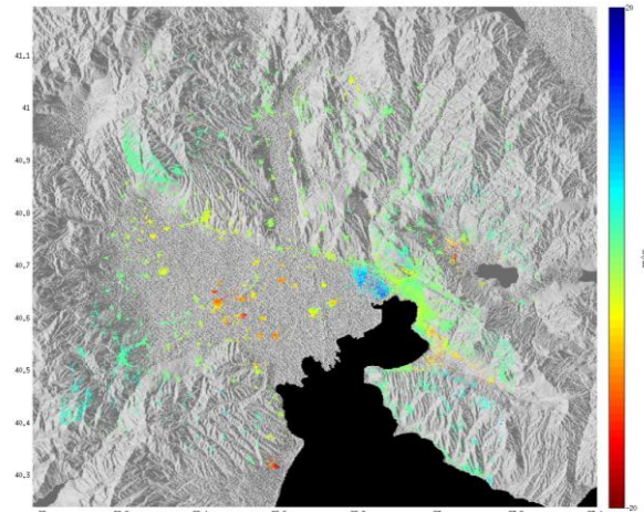
Figure 7. PS results from Envisat data (2002-2010).
