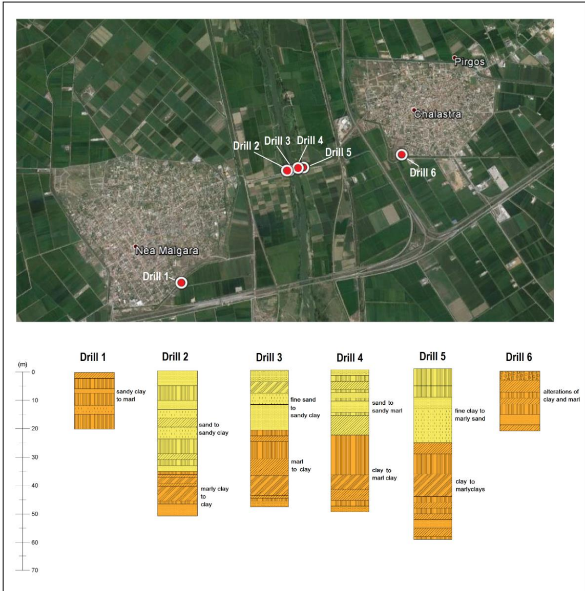
Figure 4. Drills from the area of Nea Malgara, Kimina and Chalastra. In past times the area was filled with loose material (like marls and clays) and now there is natural consolidation causing the settlement of the area.
