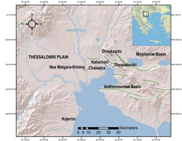
Figure 1. General view of the area of study. Green lines depict active faults. The Inset map showing Greece depicts, with the black rectangle, the area of study.
