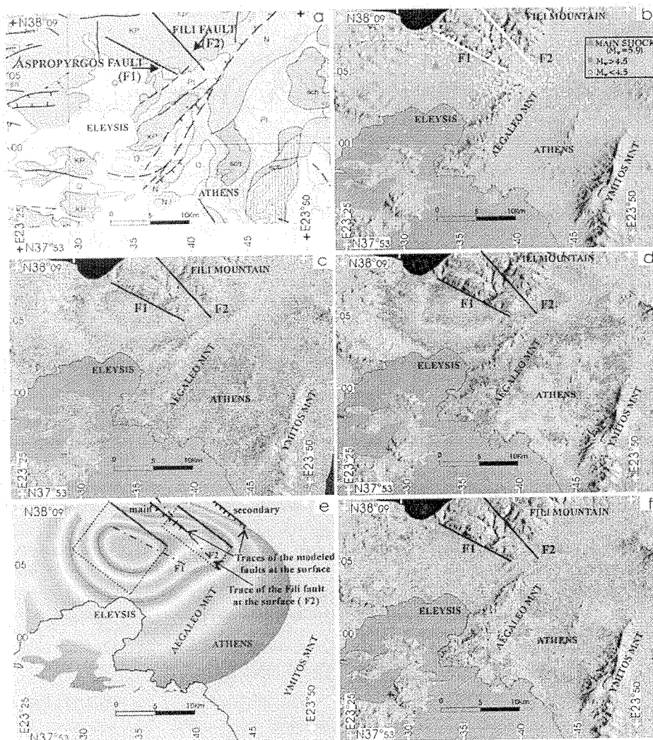
Plate 1. (a) Seismotectonic map of Athens with seismogeological elements. The Aspropyrgos (F1) and Fili (F2) faults are indicated; (b) Distribution of aftershocks recorded by the Geodynamics Institute of the National Observatory of Athens (NOA) array. (c, d) Coseismic interferograms spanning the periods [Nov. 27, 1997 to Sept. 23, 1999] and [Sept. 19, 1998 to Oct. 9, 1999]. (e) Modeled interferogram calculated by least square inversion of the fringes in Plates 1c and 1d. The two modeled fault segments and their traces on the surface, as well as the mapped Aspropyrgos (F1) and Fili (F2) faults are illustrated. (f) Preseismic interferogram spanning the period [July 22, 1995 to July 15, 1999].
