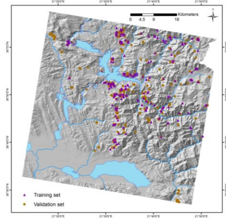
Figure 8. Landslide distribution map as location points
