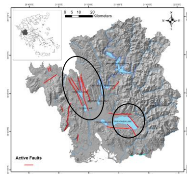
Figure 15. Active fault zones map indicating Amphilochoia fault zone (upper left) and Trichonis structure (low right)
