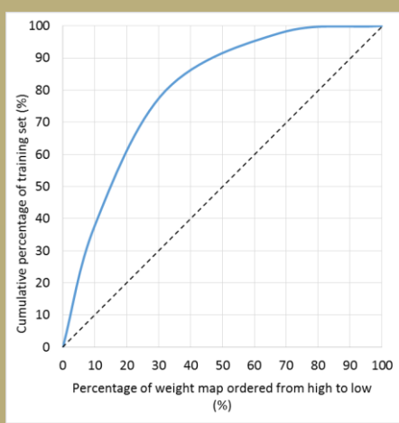
Identification of the most probable initiation areas by attributing weight values based on landslide densities for each parameter class. (Corominas et al. 2013)
