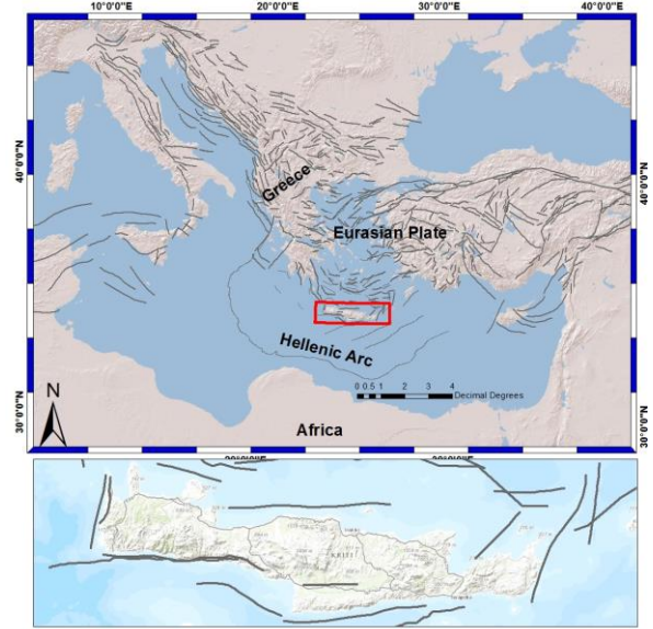
Figure 2. Fault sources map in Eastern Mediterranean and Greece. Inset shows our area of interest (red box). Grey lines represent the largest faults in the Eastern Mediterranean region ( L \geq 30\text{km} ), [8]
