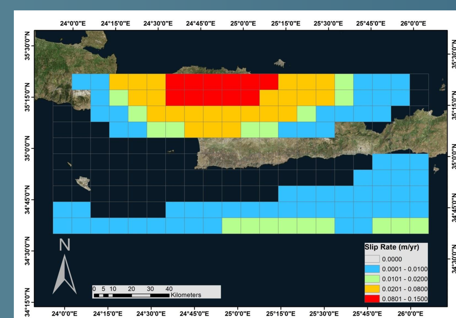
Interseismic slip rate distribution as obtained from the linear inversion for the Central part of Crete Island
