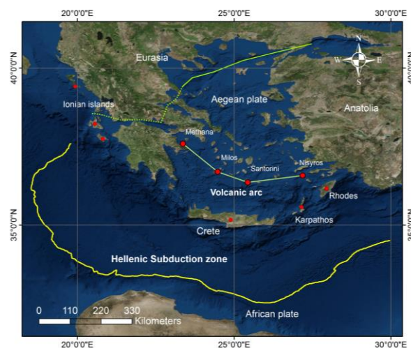
Figure 1. Map of the Aegean region showing the surface projection of the Hellenic arc, relative location of the Aegean and Anatolian plates and the volcanic and non-volcanic arc island.
