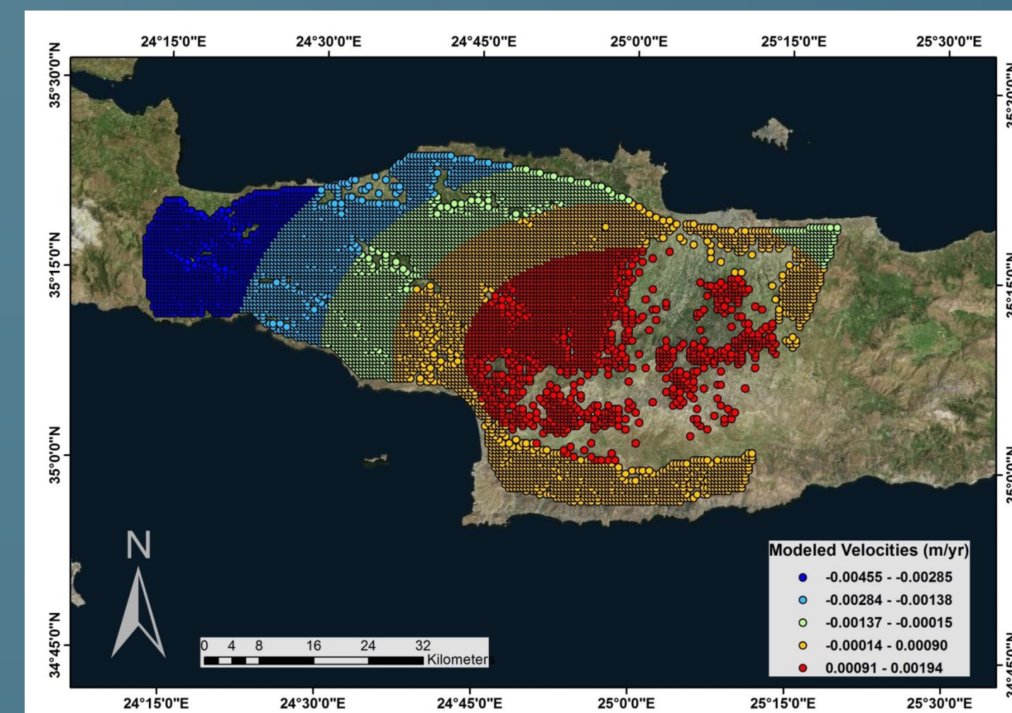
Modelled velocities of central Crete
