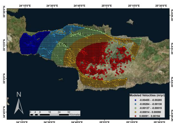
Figure 12. Modelled velocities over central Crete.
