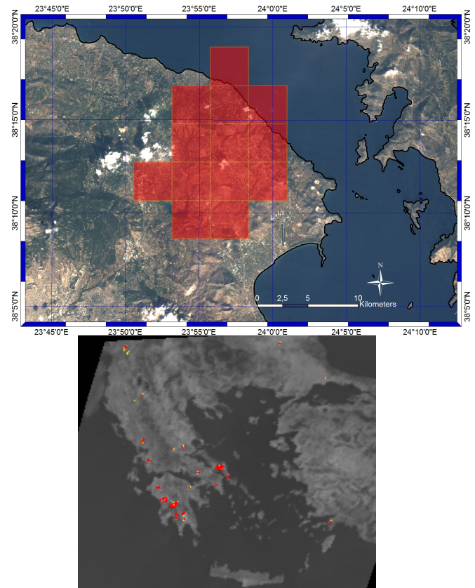
Figure 2. (top) Vector hotspot layer depicting fires that occurred in 2009 at northeastern Attica, and (bottom) raster overview of the 2007 Peloponnesus forest wildfires. Red pixels correspond to 'fires', whereas yellow to 'potential fires'.
